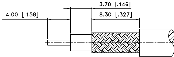
RECOMMENED CABLE STRIPPING DIM'S
