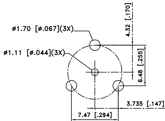
PCB MOUNTING HOLES
