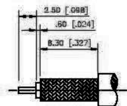
RECOMMENDED CABLE STRIPPING DIMENSIONS
