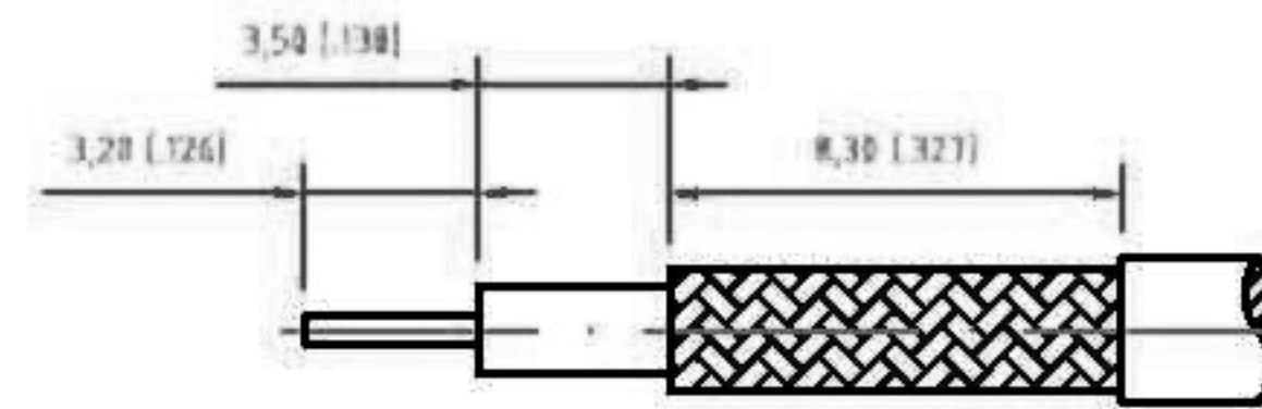
RECOMMENDED CABLE STRIPPING DIM'S
