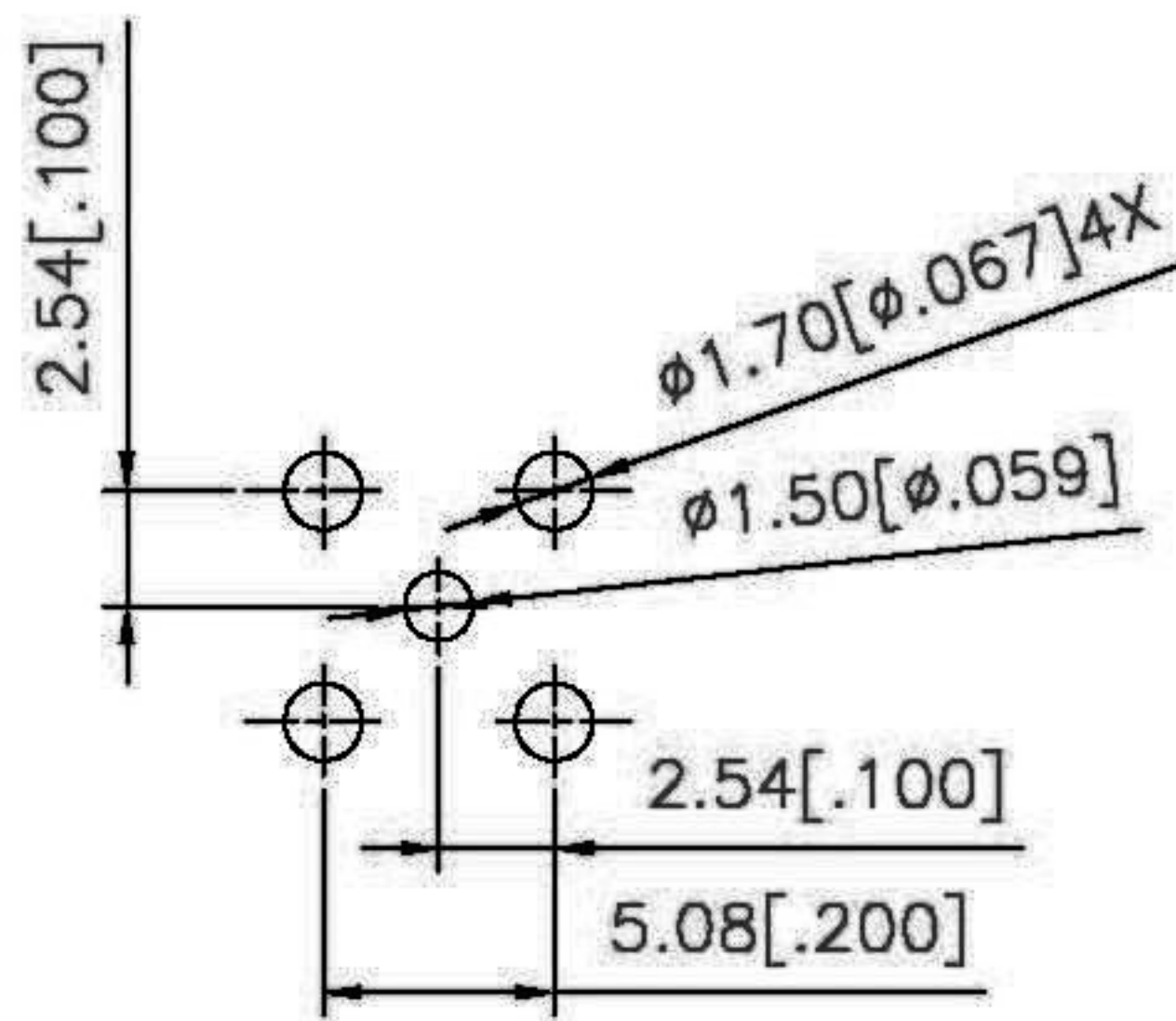
PCB MOUNTING HOLES
