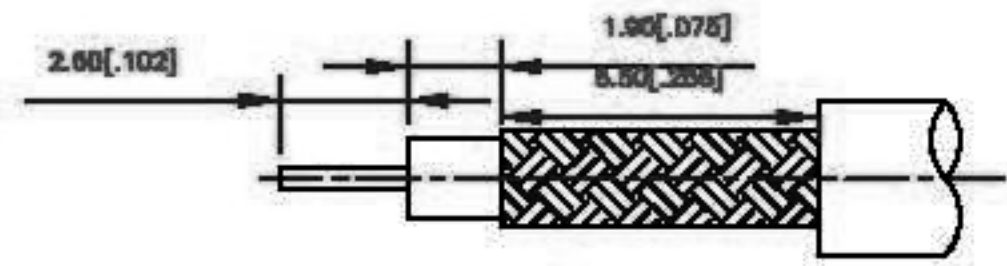
RECOMMENDED CABLE STRIPPING
