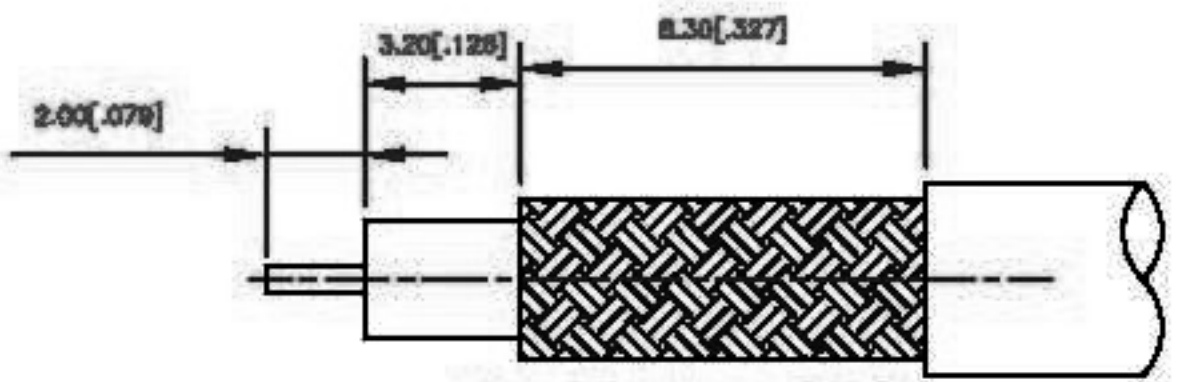
RECOMMENDED CABLE STRIPPING DIM'S
