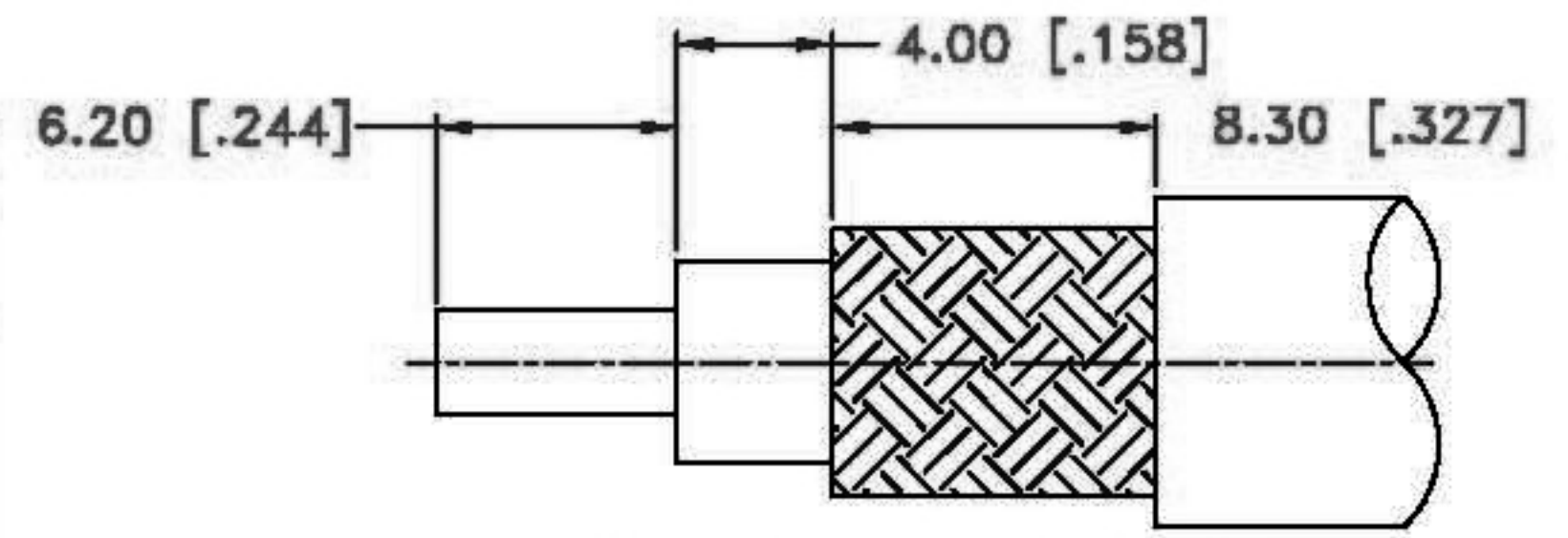
RECOMMENDED CABLE STRIPPING DIM'S
